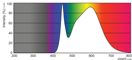
TLED STD 900 mm 15 W /840 T8 C
