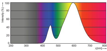
LEDtube HF 1200mm HO 18W /830 T8
